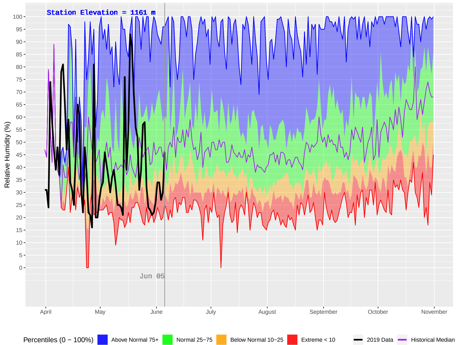
TIMOTHY (234) : Historical (1990–2018) and Current (2019) Daily Relative Humidity
