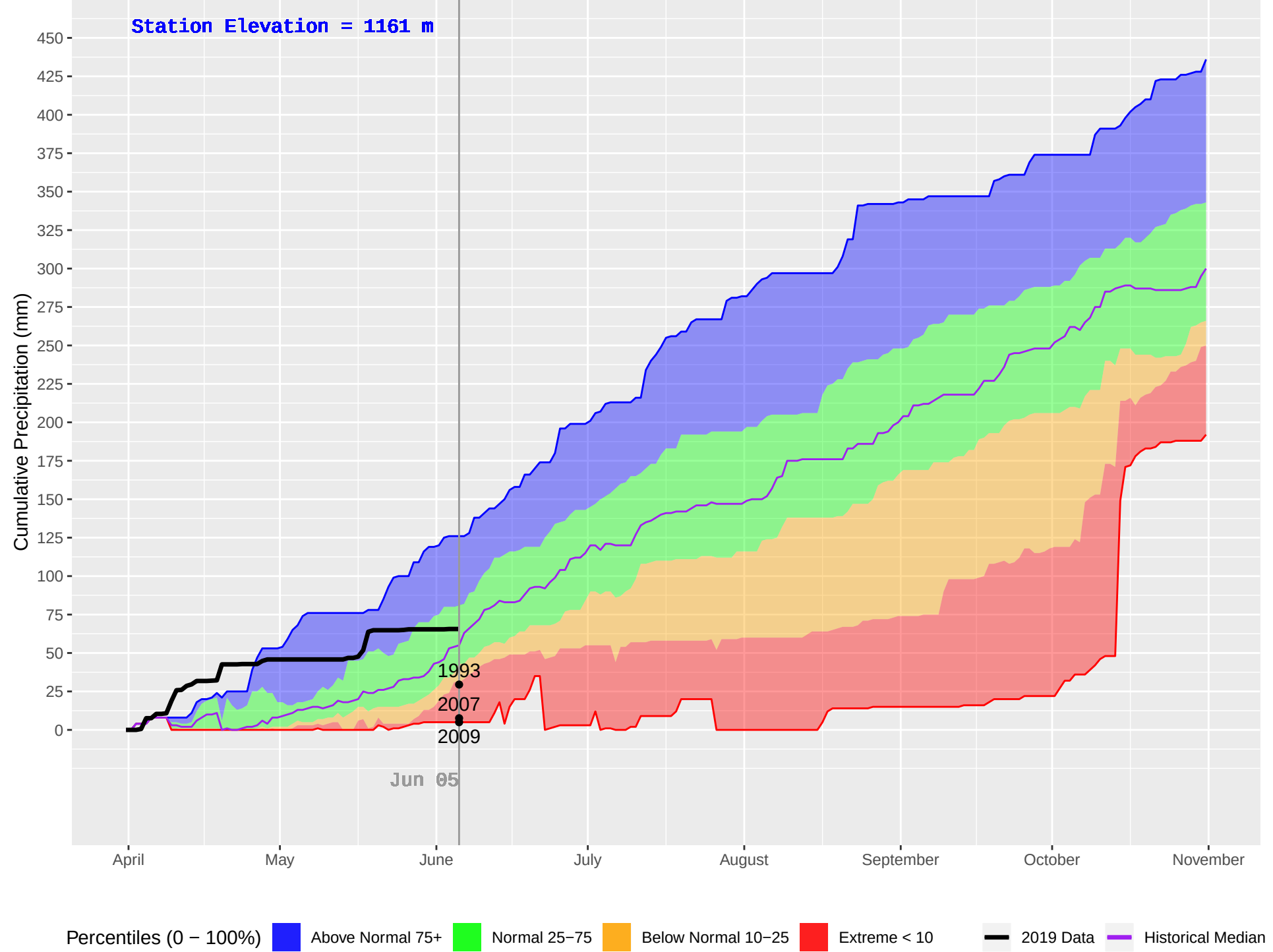
TIMOTHY (234) : Historical (1990–2018), Current (2019) Daily Cumulative Precipitation
