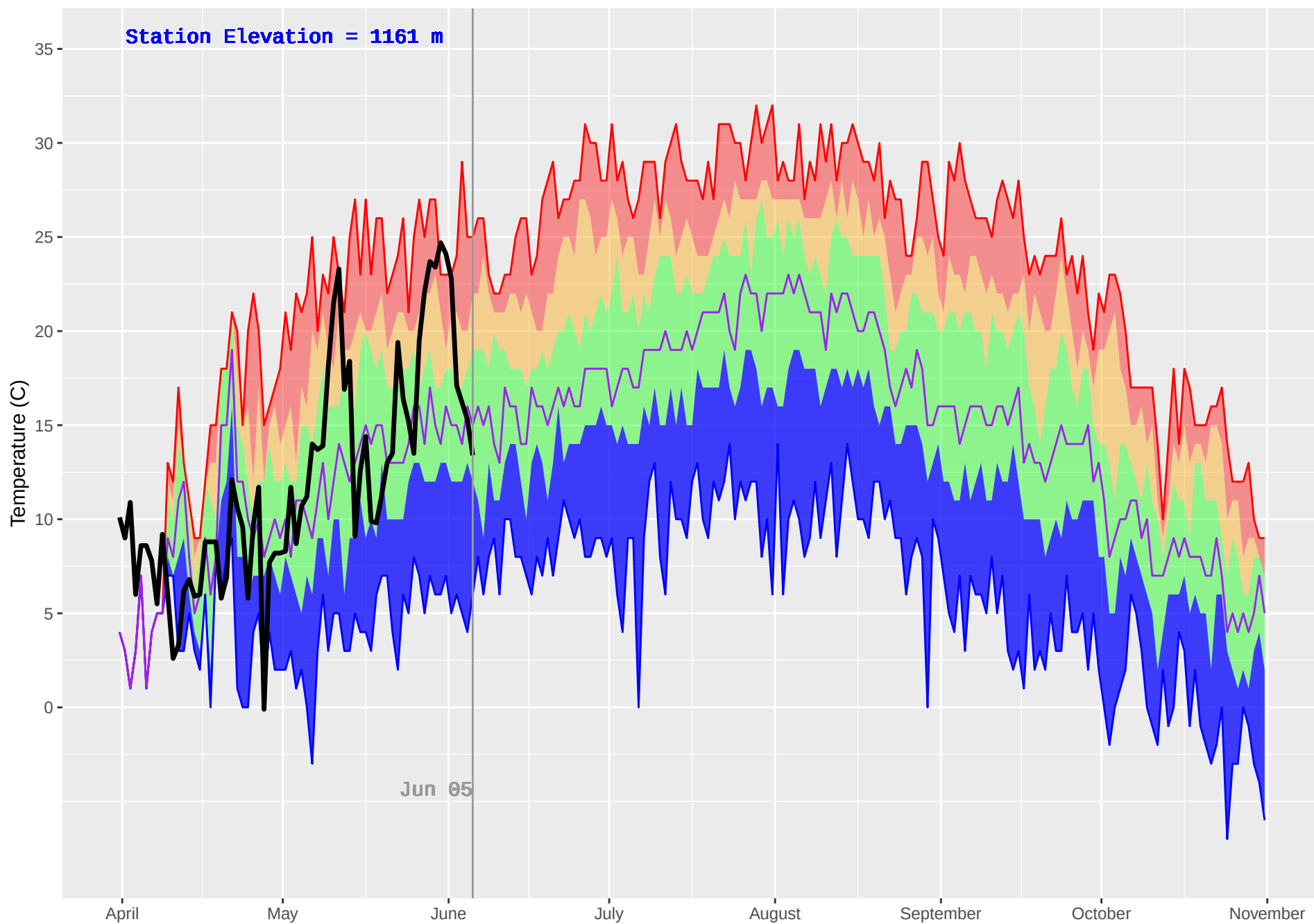
TIMOTHY (234) : Historical (1990–2018) and Current (2019) Daily Temperature
