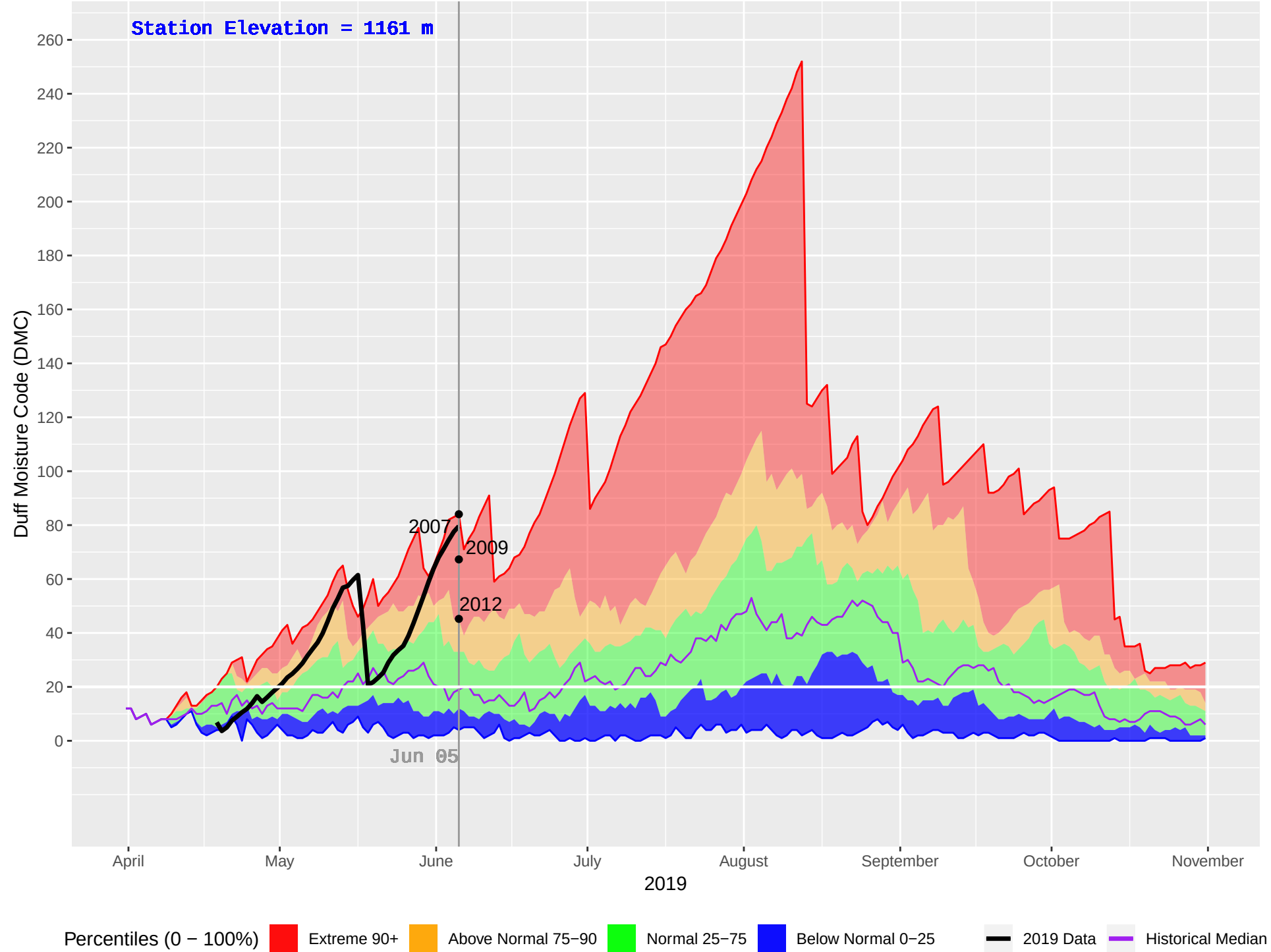
TIMOTHY (234) : Historical (1990–2018), Current (2019) Daily Duff Moisture Code (DMC)
