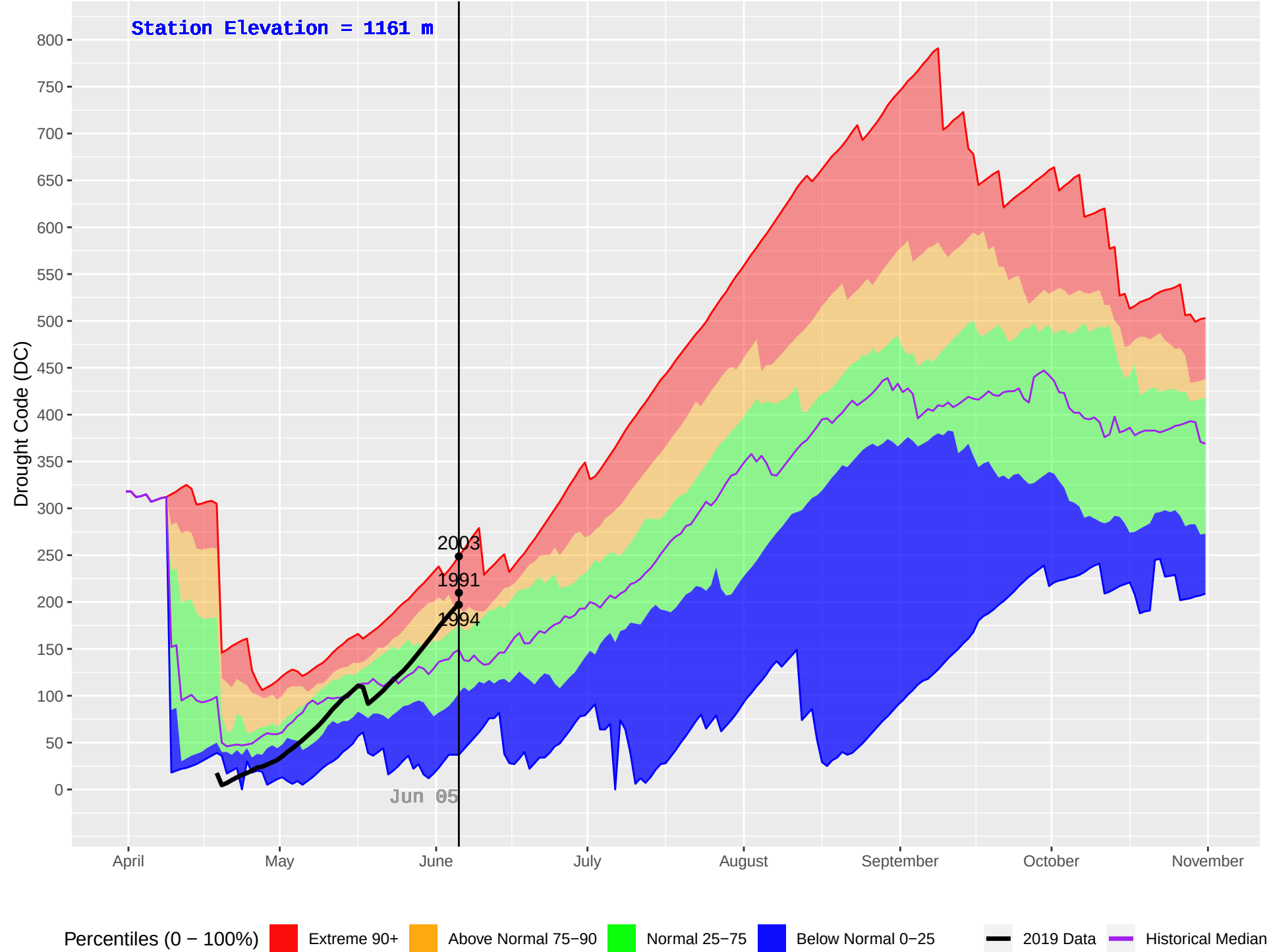
TIMOTHY (234) : Historical (1990–2018) and Current (2019) Daily Drought Code (DC)
