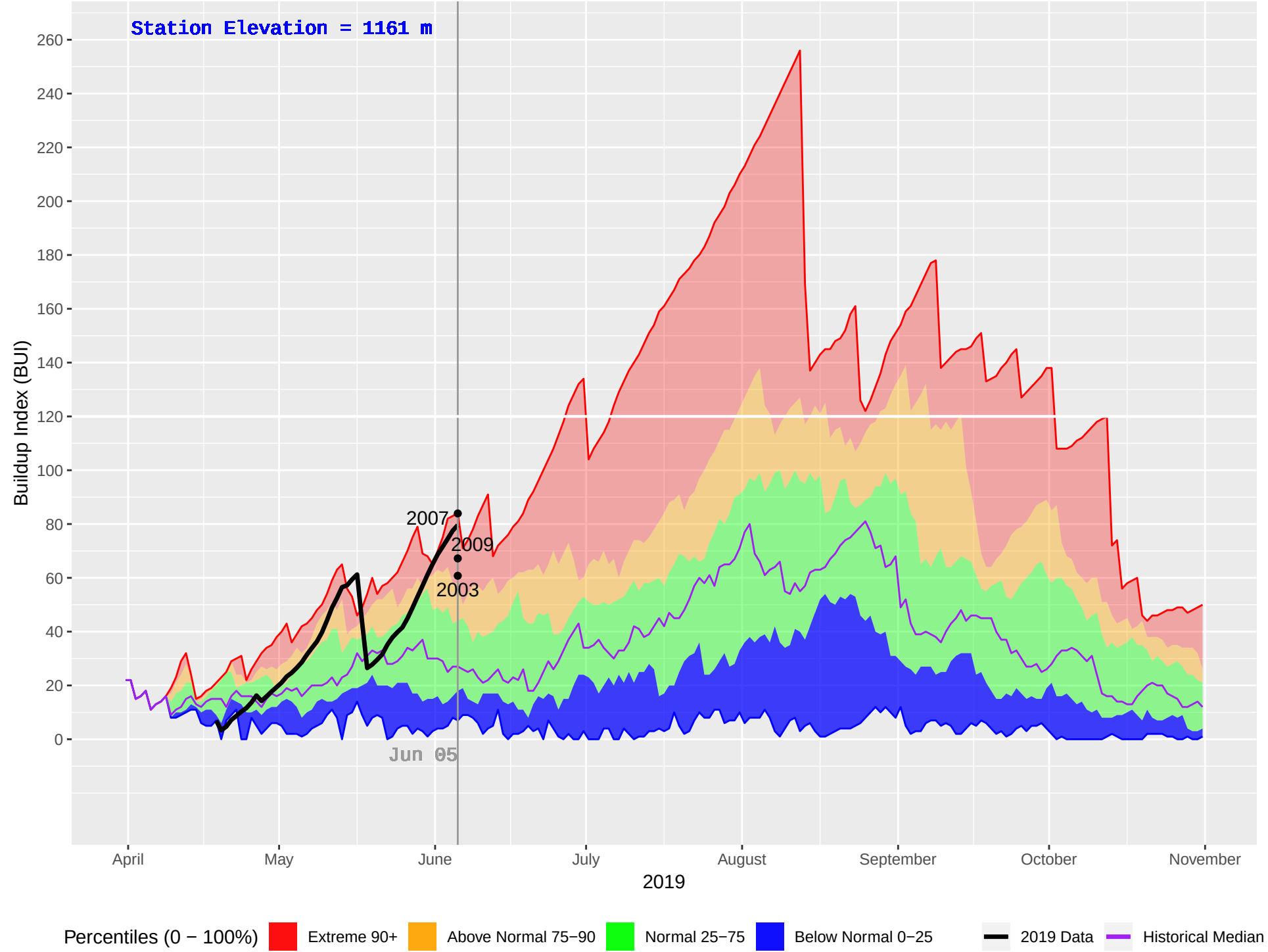
TIMOTHY (234) : Historical (1990–2018), Current (2019) Daily Buildup Index (BUI)
