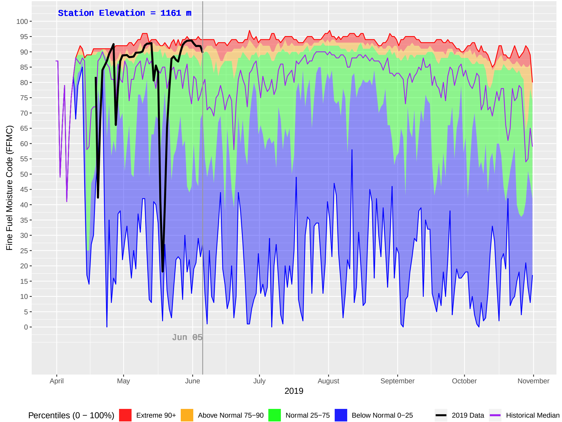
TIMOTHY (234) : Historical (1990–2018) and Current (2019) Daily Fine Fuel Moisture Code (FFMC)
